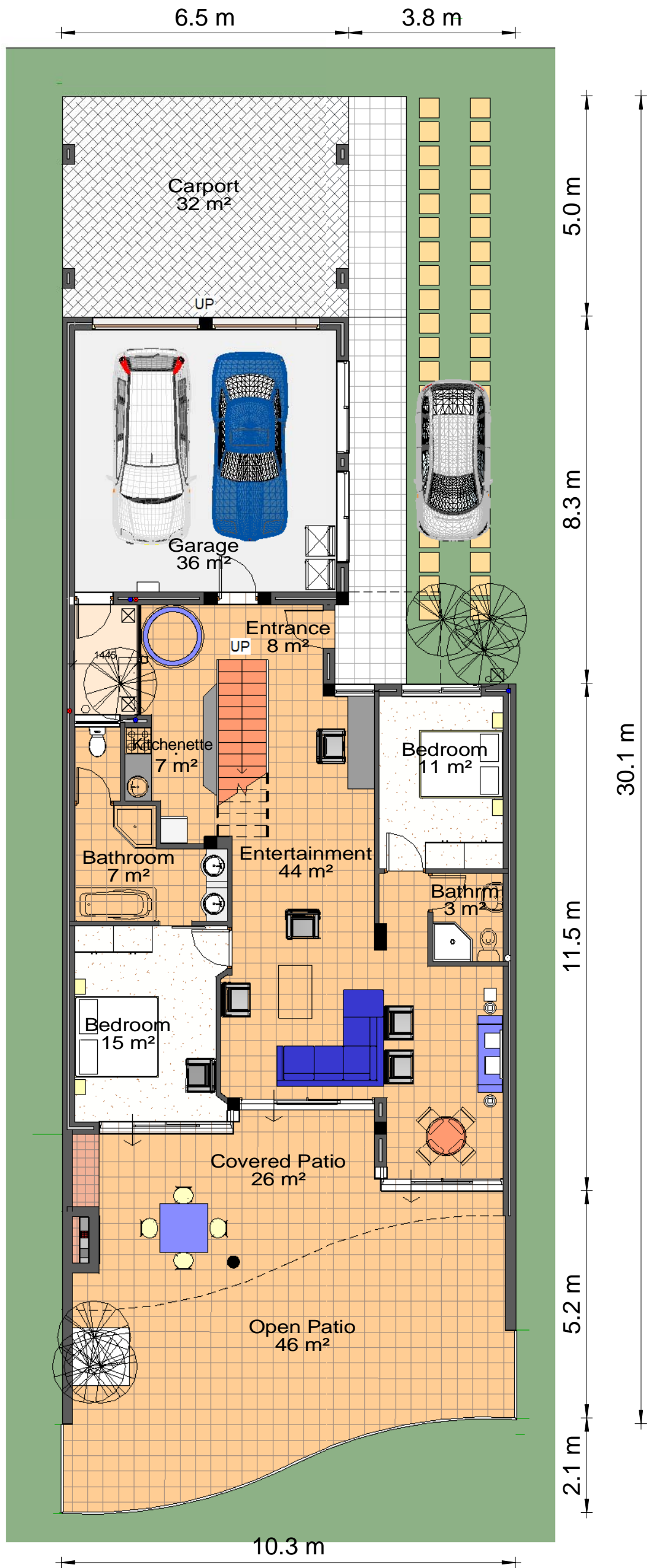
OCEAN VILLA 2 STOREY UNIT GROUND FLOOR PLAN
