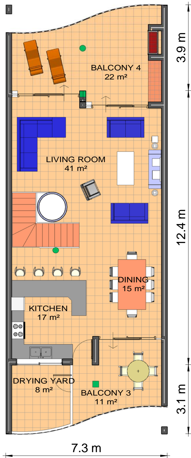
LAGOON TERRACE 3 STOREY UNIT 2ND FLOOR PLAN
