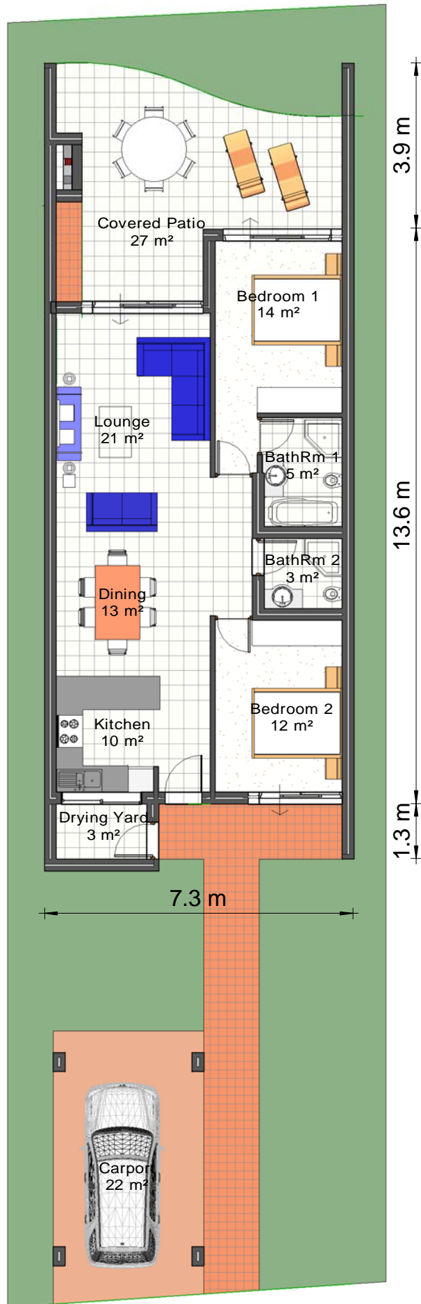
LAGOON TERRACE SINGLE STOREY UNIT GROUND FLOOR PLAN
