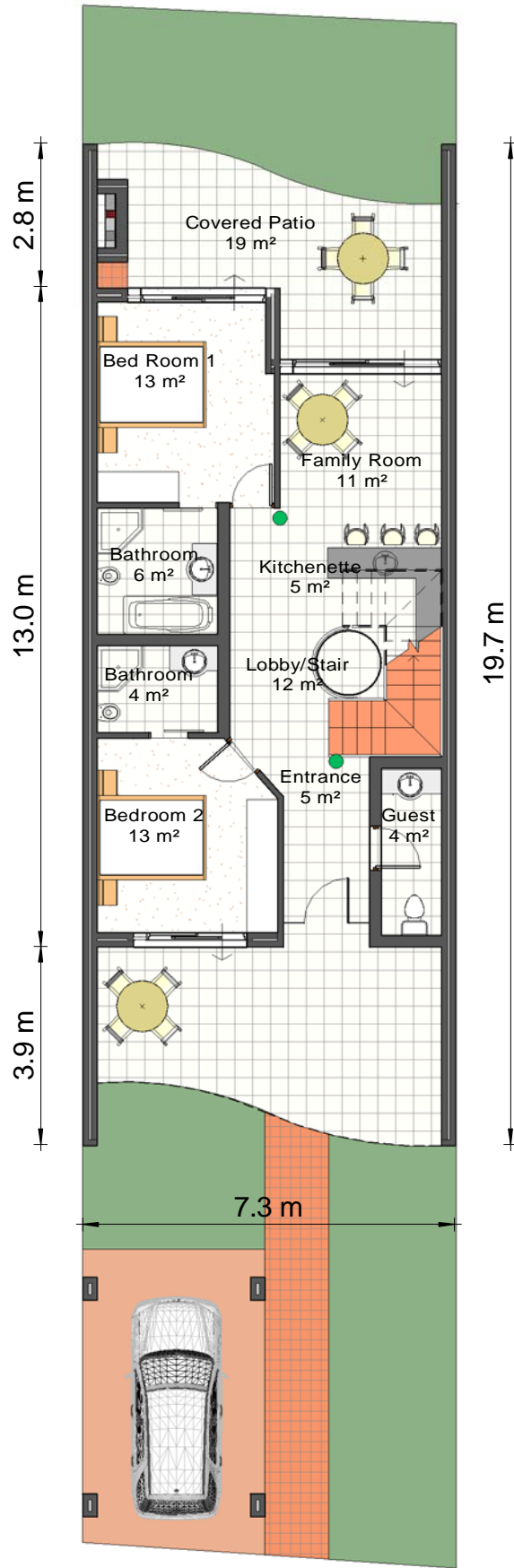
LAGOON TERRACE 2 STOREY UNIT GROUND FLOOR PLAN
